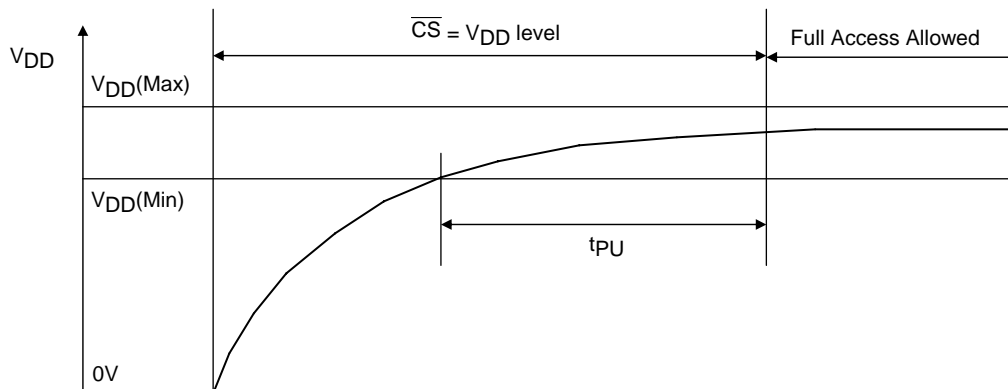
Figure 18 Power-on Timing
