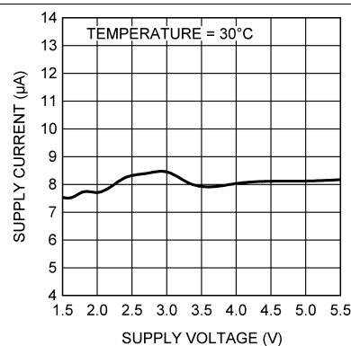
Figure 6. Supply Current vs Supply Voltage
