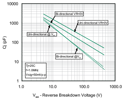
Figure 5 - Typical Junction Capacitance Uni-Directional
