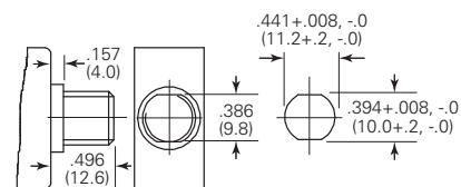
Option 3 & 6 – M11 X 1.0 Thread
