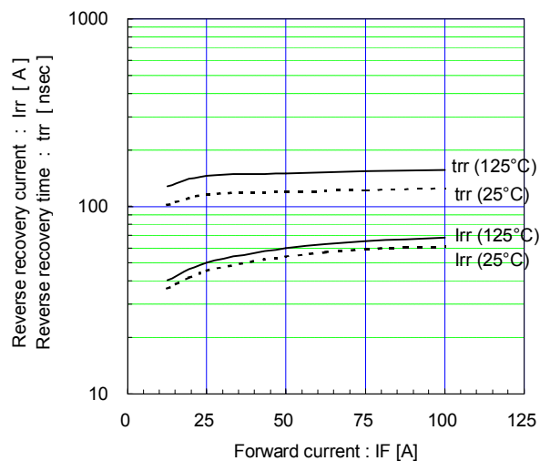
[ Inverter ] Reverse recovery characteristics (typ.) Vcc=600V, VGE=±15V, Rg=9.1Ω
