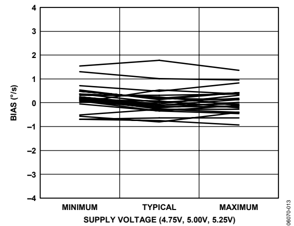
Figure 8. Bias vs. Supply Voltage
