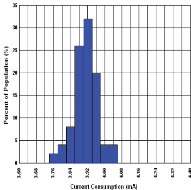
Figure 5.20 Current Consumption at +25°C
