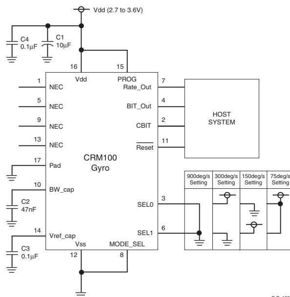
Figure 7.3 Peripheral Circuit - Analogue Output (CRM100)
