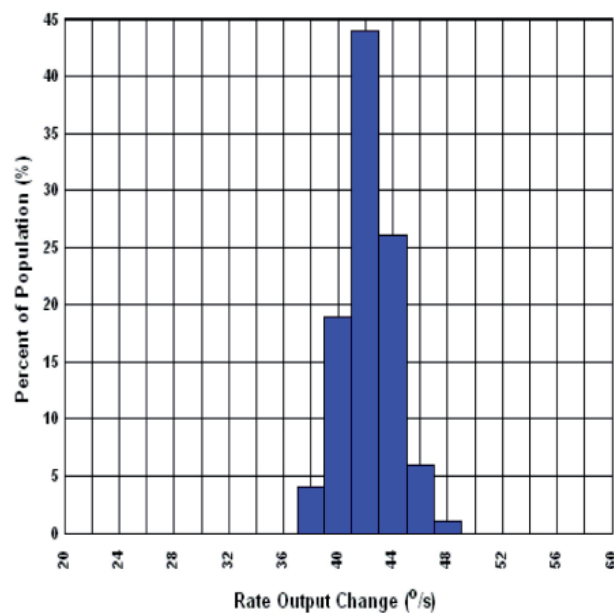
Figure 5.39 Rate Output Change with Digital CBIT at +25°C
