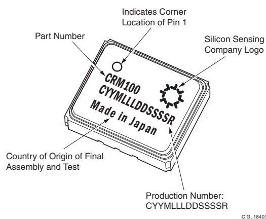
Figure 11.1 Part Marking
