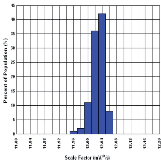
Figure 5.14 Analogue Scale Factor at +25°C
