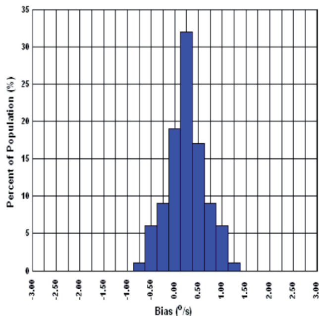
Figure 5.32 Digital Bias at +25°C
