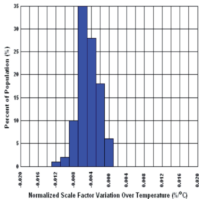
Figure 5.35 Normalized Digital Scale Factor Variation Over Temperature
