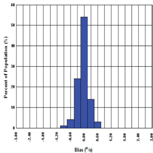
Figure 5.12 Analogue Bias at +25°C
