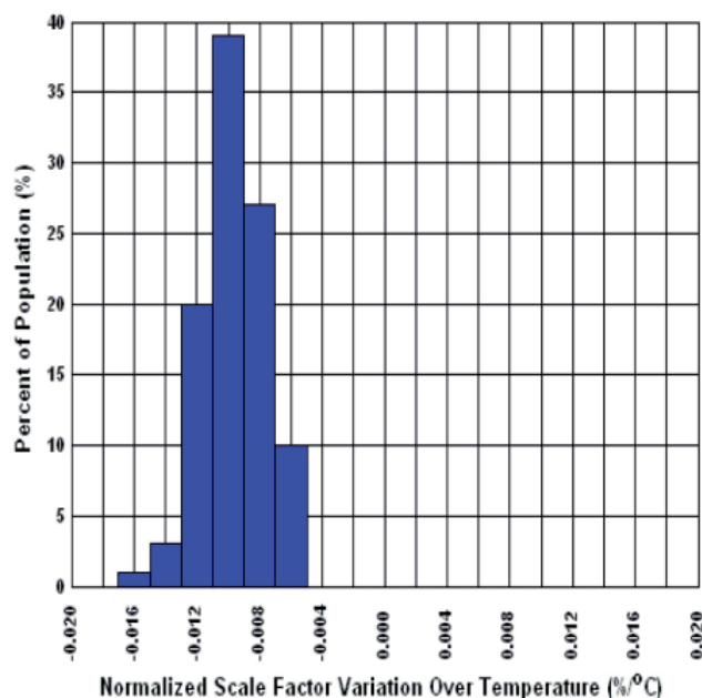
Figure 5.15 Normalized Analogue Scale Factor Variation Over Temperature
