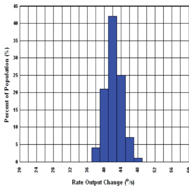
Figure 5.19 Rate Output Change with Analogue CBIT at +25°C
