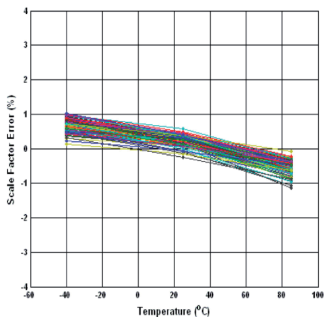
Figure 5.3 Analogue Scale Factor Error (12 mV/°/s nominal) vs Temperature
