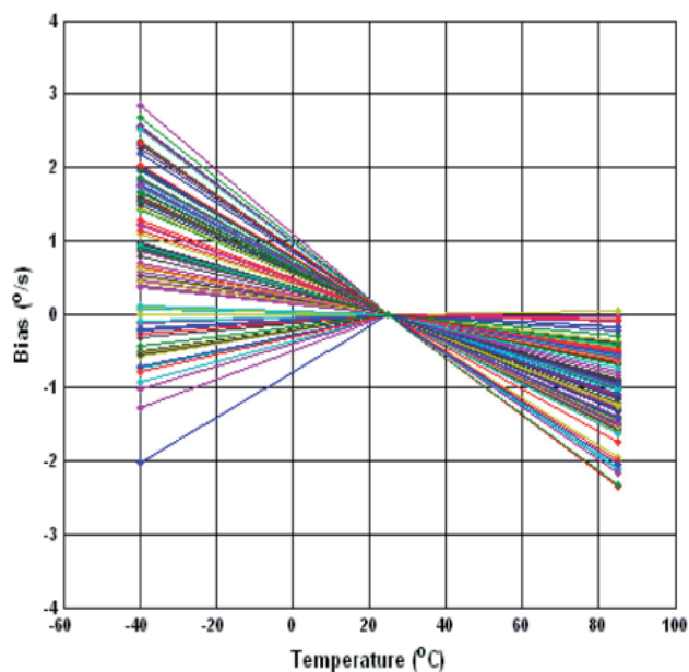
Figure 5.2 Normalized Analogue Bias vs Temperature
