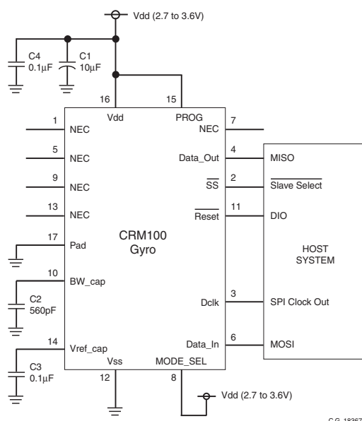
Figure 7.4 Peripheral Circuit - Digital Output (CRM100)
