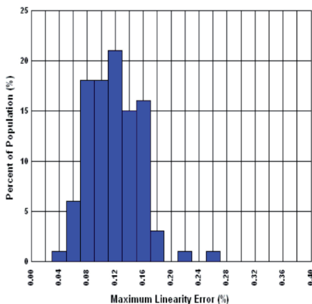
Figure 5.38 Digital Output Maximum Linearity Error at +85°C (Best Straight Line Fit)
