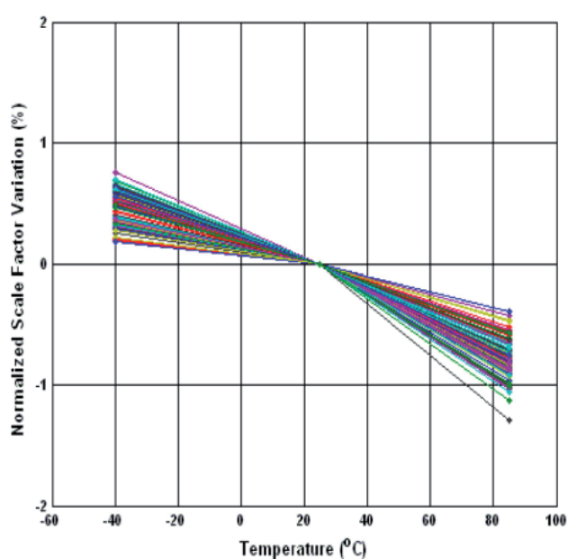
Figure 5.4 Normalized Analogue Scale Factor Variation vs Temperature
