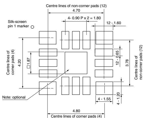
Figure 7.2 Recommended Pad Layout (CRM100)
