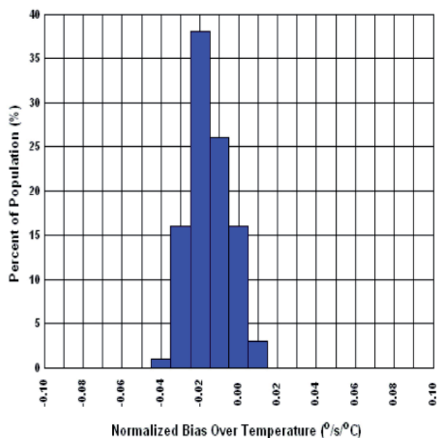
Figure 5.13 Normalized Analogue Bias Over Temperature
