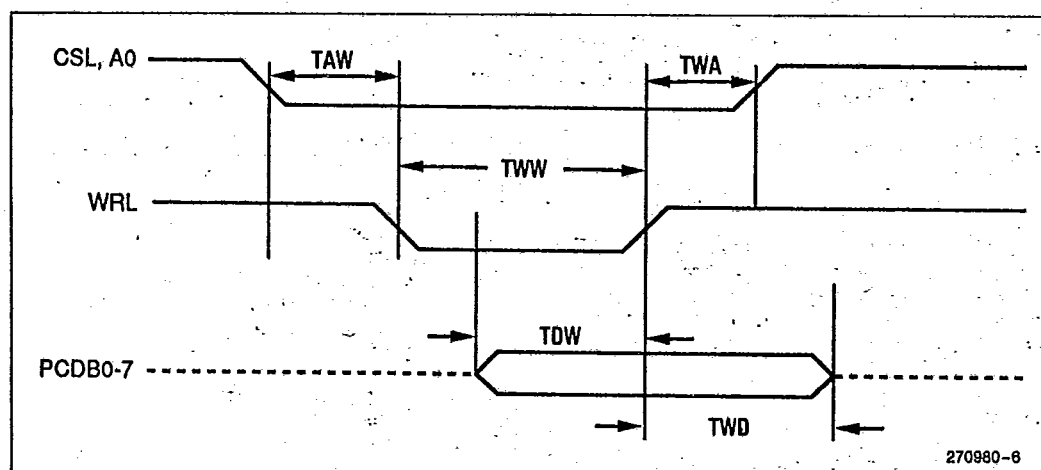
Figure 17. Host-Interface Write
