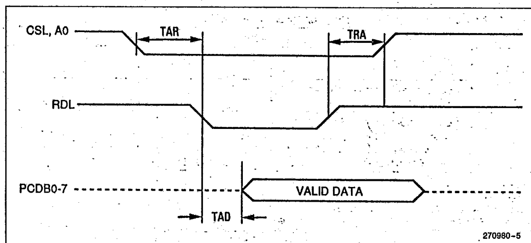
Figure 16. Host-Interface Read
