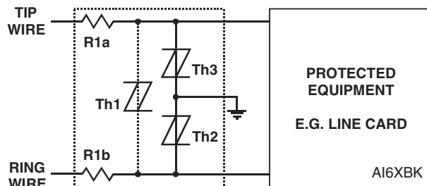
Figure 15. Protection Module
