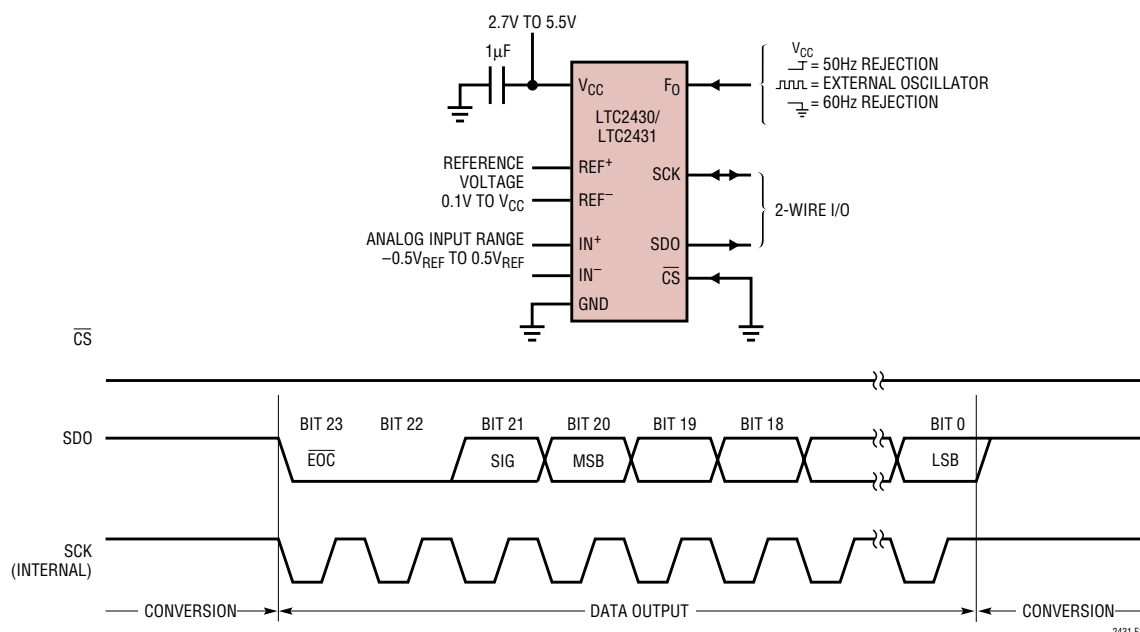
Figure 10. Internal Serial Clock, \overline{\text{CS}} = 0 Continuous Operation
