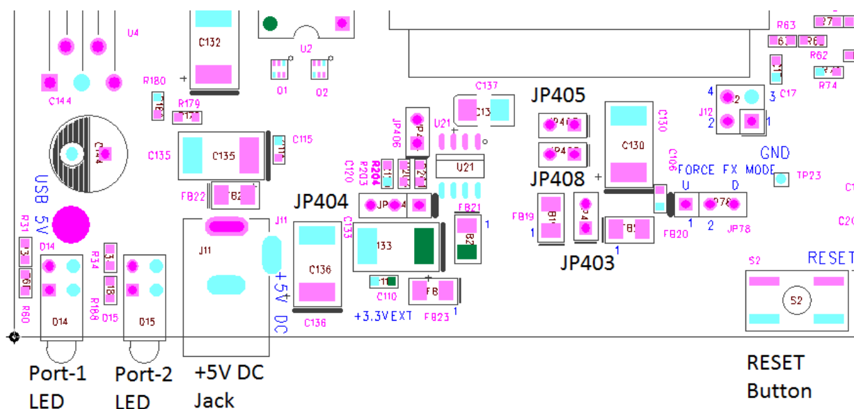
Figure 2 Power Supply Section and Related Jumper Locations
