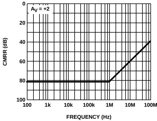
FIGURE 21. CMRR
