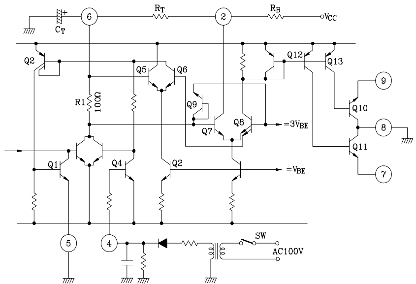
Fig.1 Charge and Discharge Level Equivalent Circuit
