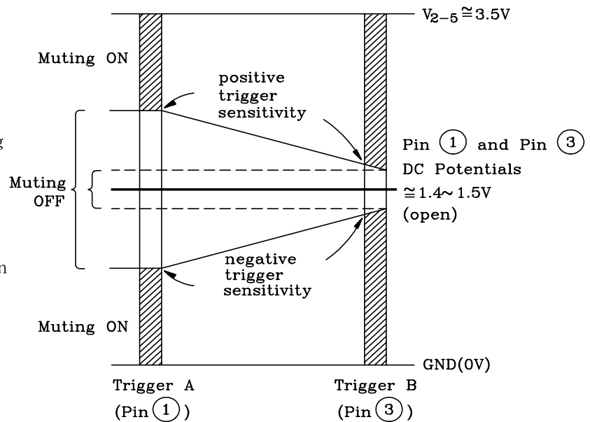
Fig.5 Trigger Level
