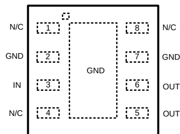
WSO (NGN) Package 8 Pins Top View
