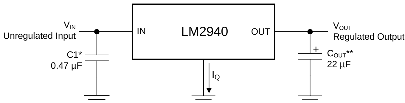
Simplified Schematic
