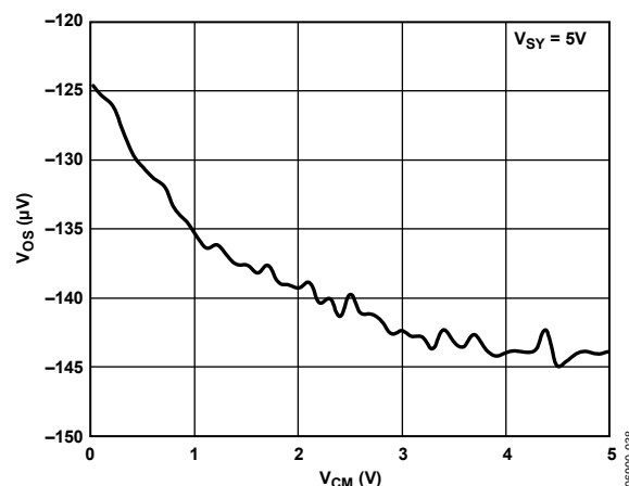
Figure 16. Input Offset Voltage vs. Input Common-Mode Voltage
