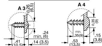
Barbed inserts
