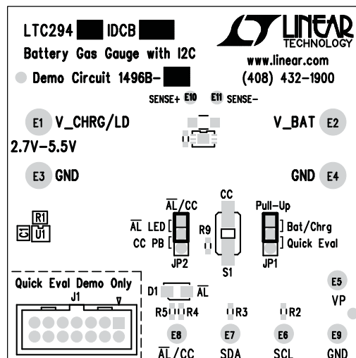
Figure 1. DC1496B
