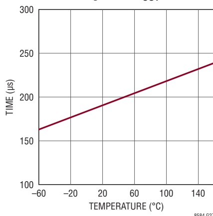
OUT Pin Amplifier 1% Settling Time, C_{OUT} = 220\text{nF}
