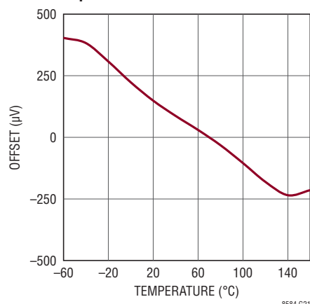
V_{SNS} Amplifier Input Referred Offset
