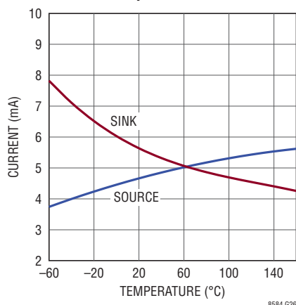
OUT Pin Amplifier Drive Current
