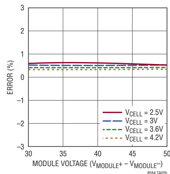
Typical Current Measurement Error
