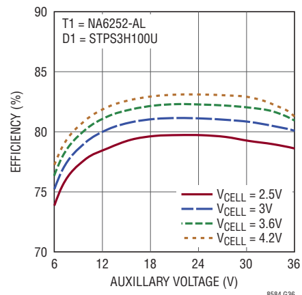
Conversion Efficiency
