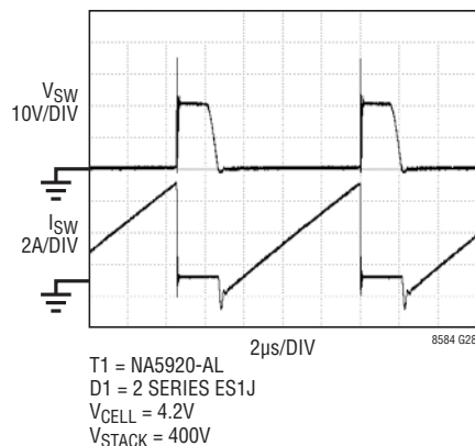
Switching Waveform
