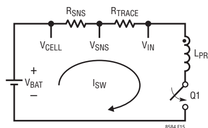
Figure 15. R_{TRACE} Minimization
