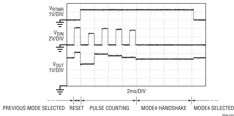
Figure 20. Typical Serial Mode Communication Waveforms
