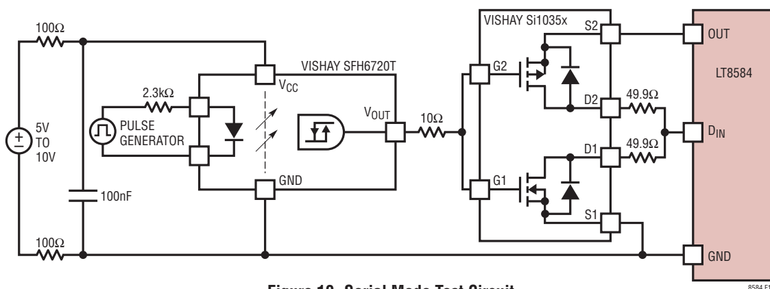
Figure 19. Serial Mode Test Circuit
