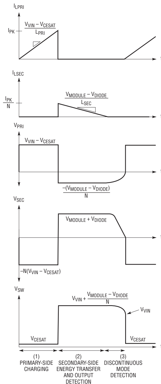
Figure 1. Simplified Discharging Waveforms
