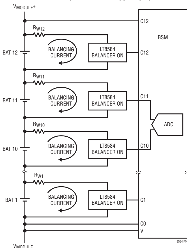
TWO-WIRE BATTERY CONNECTION
