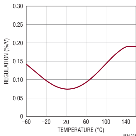
Handshake Voltage Line Regulation
