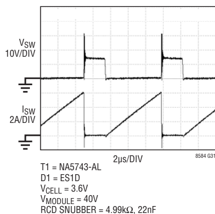
Switching Waveform
