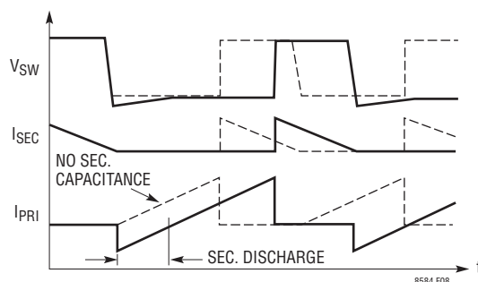
Figure 8. Effect of Secondary Winding Capacitance
