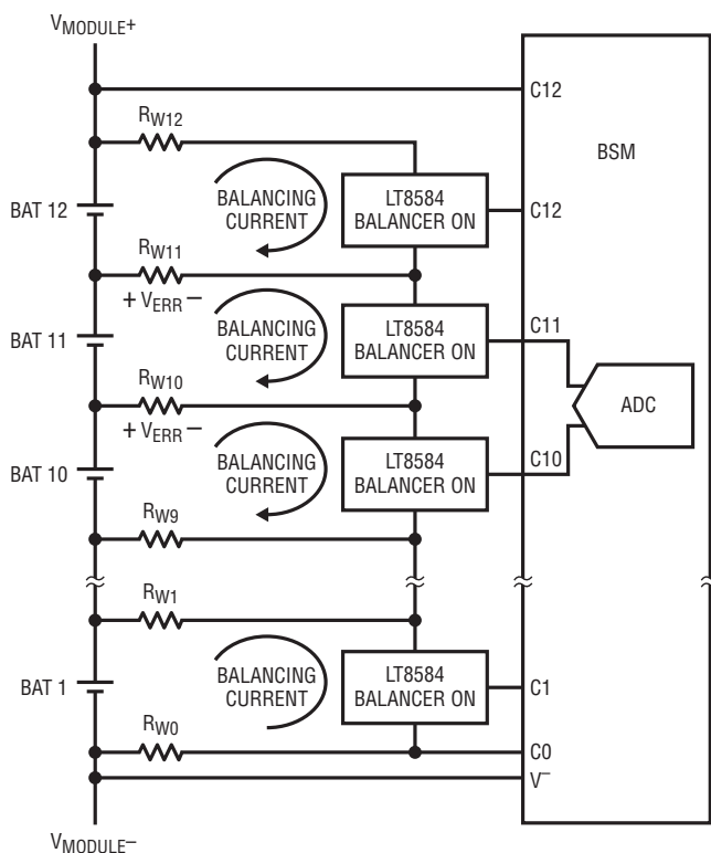
Figure 16. LT8584 Battery Connections
