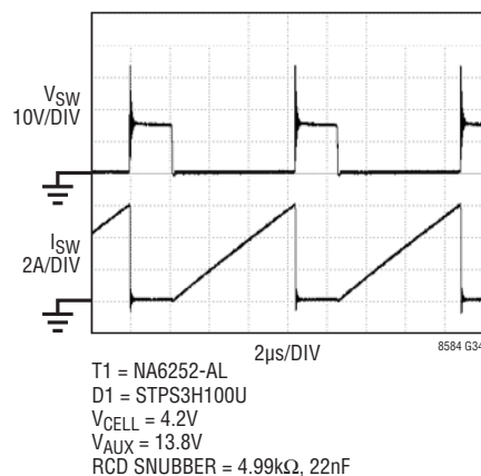
Switching Waveform
