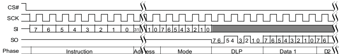
Figure 88. DDR Fast Read Initial Access (4-Byte Address, 0Eh or 0Dh [ExtAdd=1], EHPLC=01b)
