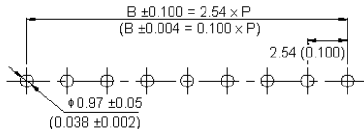
PCB Layout
