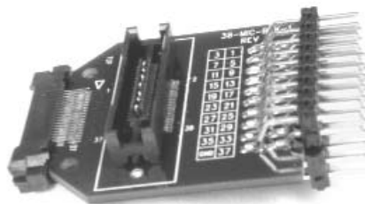
MICTOR Signal Monitoring Adapter
