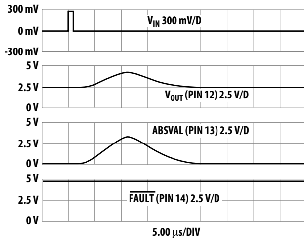
Figure 17. \overline{FAULT} rejecting a 1 \mu s, 0 V to 2 V to 0 V input. Rejection is independent of amplitude
