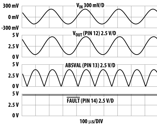
Figure 19. Sine response 400 mV peak-to-peak 4 kHz input, at V_{REF} = 5 V
