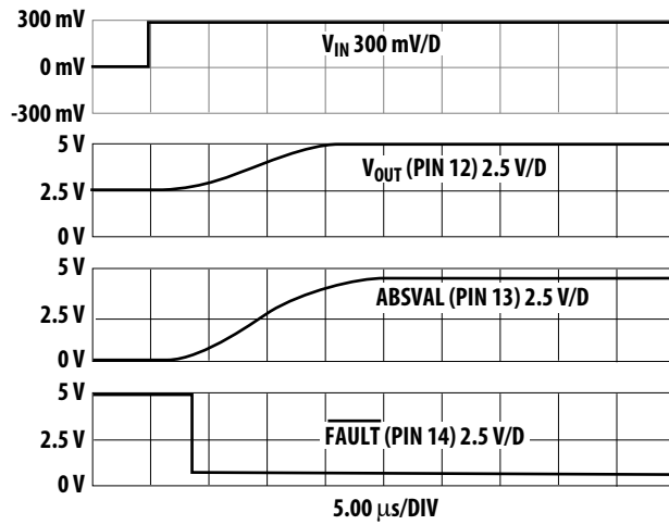
Figure 15. \overline{FAULT} detection, 0 mV to 300 mV input, at V_{REF} = 5 V
