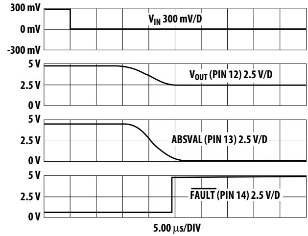
Figure 16. \overline{FAULT} release, 300 mV to 0 mV input, at V_{REF} = 5 V
