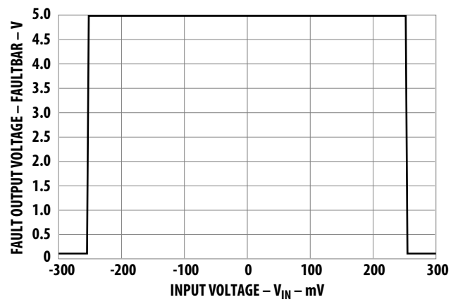
Figure 10. \overline{\text{FAULT}} output voltage vs. V_{IN}
