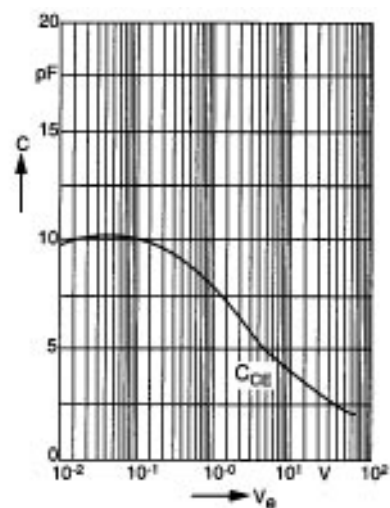
Figure 19. Transistor capacitance C=f(V_O) ( T_A=25^\circ\text{C} , f=1\text{ MHz} )
