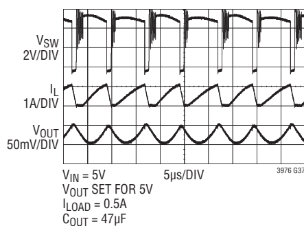
Dropout Switching Waveforms
