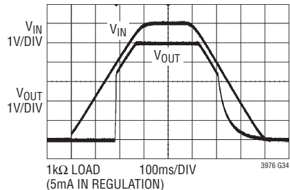
Start-Up/Dropout Performance
