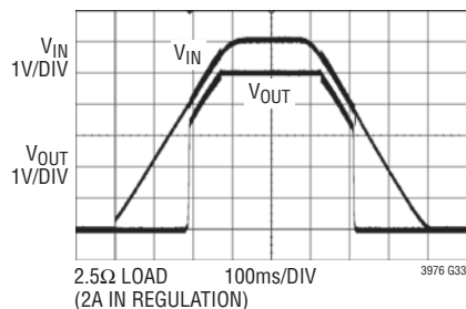
Start-Up/Dropout Performance
