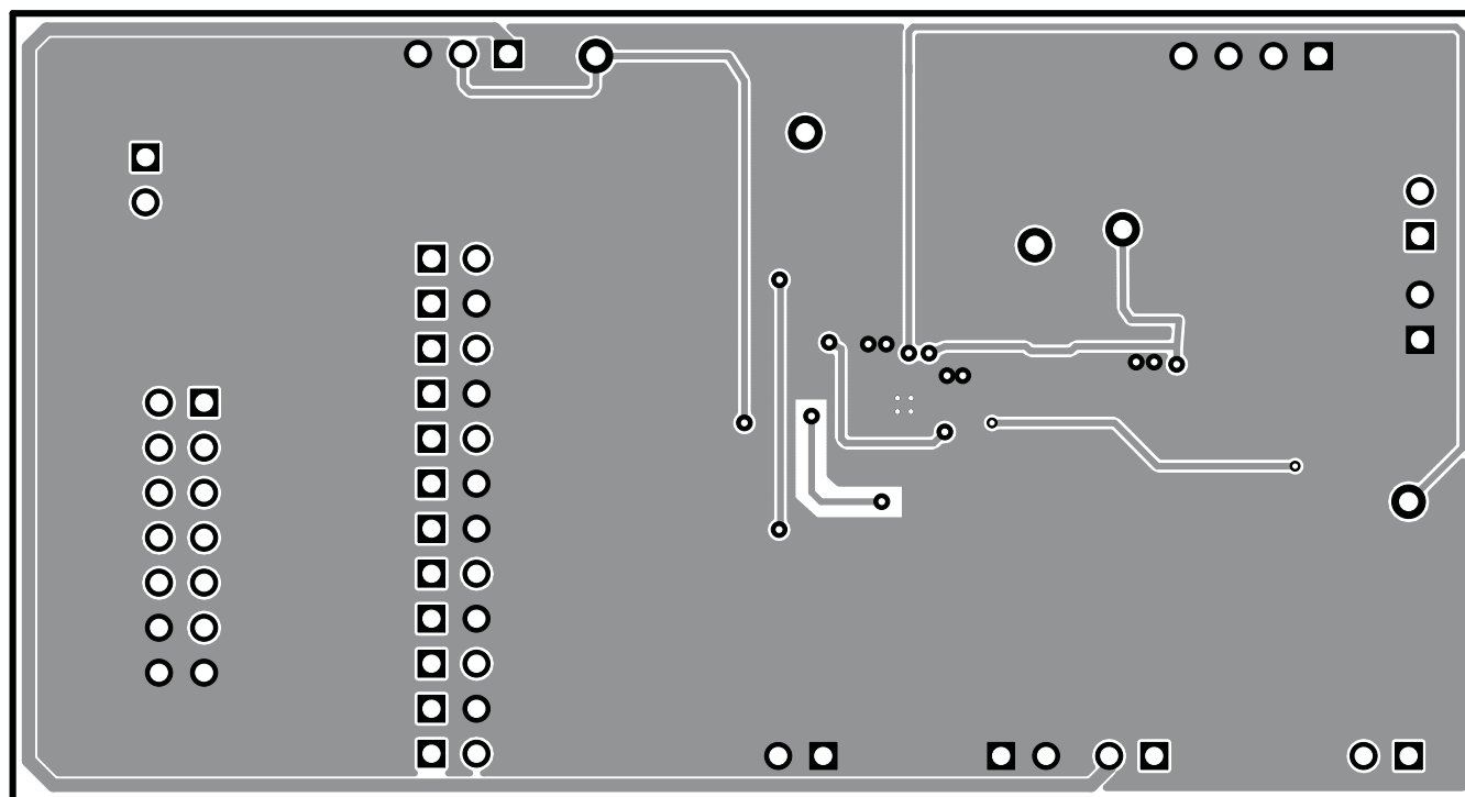
Figure 8. Bottom Layer
