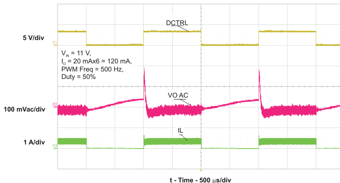
Figure 5. Output Ripple at PWM Dimming with C_O = 4.7\text{ }\mu\text{F}
