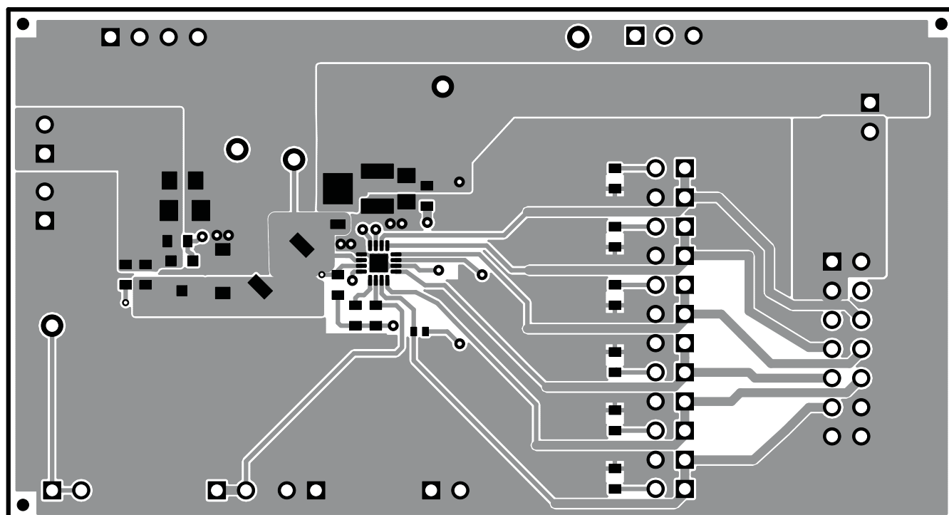
Figure 7. Top Layer
