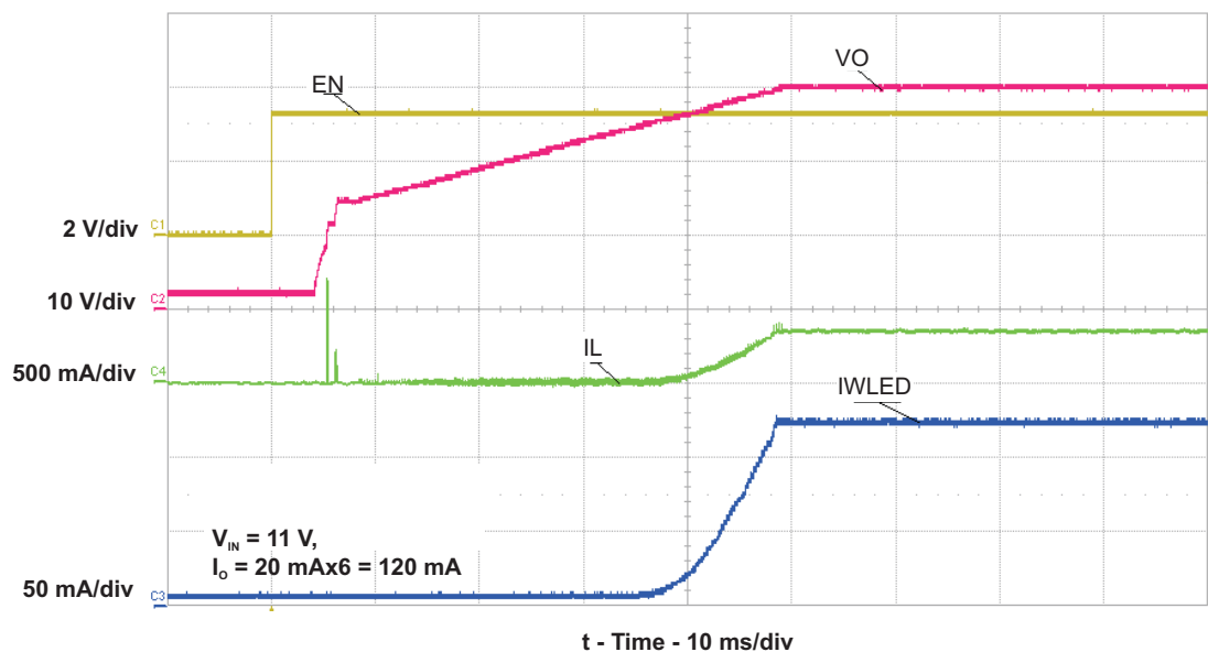
Figure 3. Start-up
