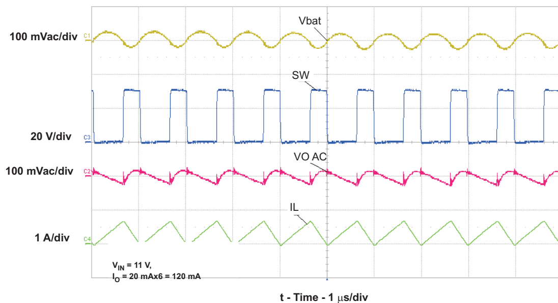
Figure 4. Switching Waveform
