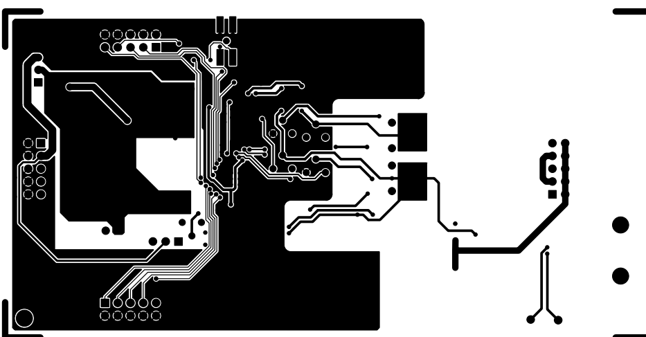
Figure 24. Si321xM-FM-DCI-EVB with Discretes Secondary Side
