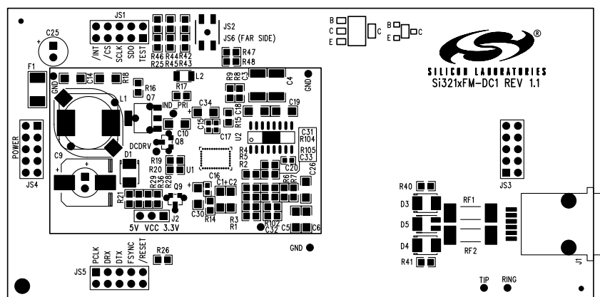
Figure 4. Si321xFM-DC1-EVB with Si3201 Primary Assembly
