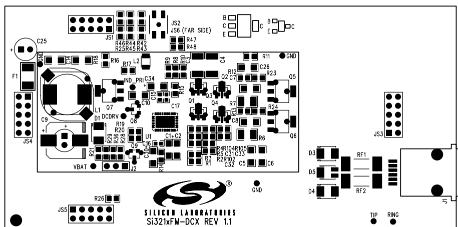
Figure 10. Si321xFM-DCX-EVB with Discretes Primary Assembly
