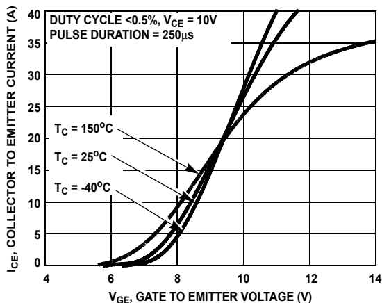
Figure 1. TRANSFER CHARACTERISTICS
