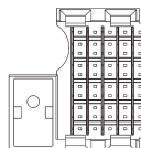
Part Number 120668 50 Position Left Shroud ESD/HDI Guide Pin
