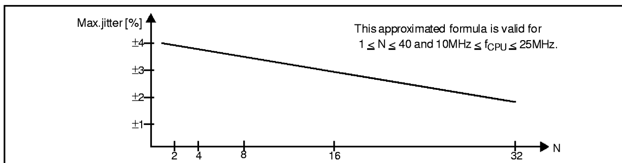
Figure 19 : Approximated maximum PLL jitter
