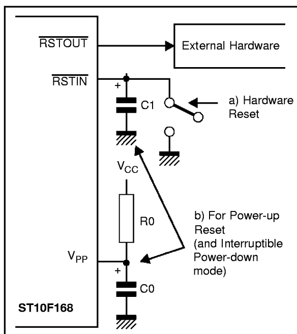
Figure 12 : Minimum External Reset Circuitry
