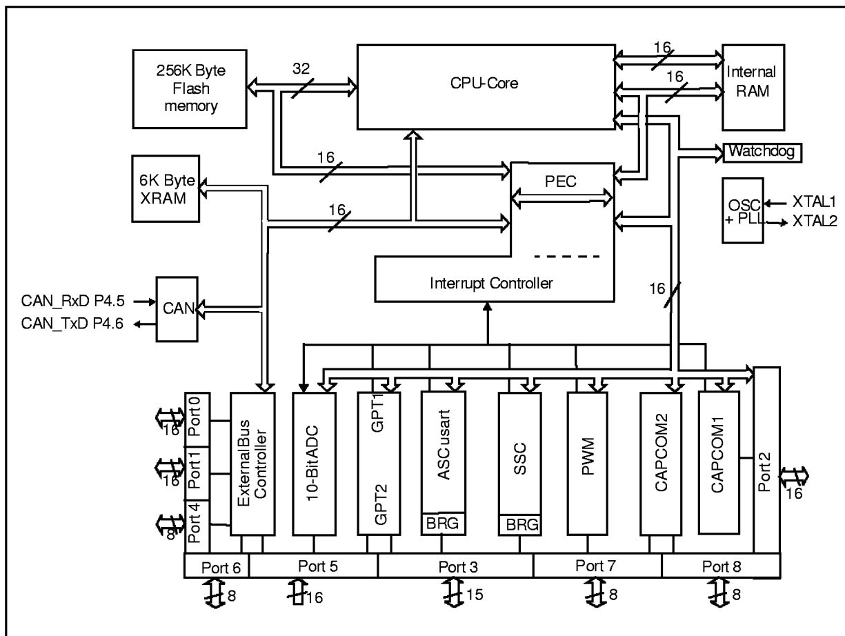
Figure 3 : Block Diagram
