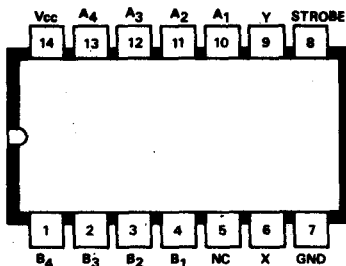
C13 DM8200N 4-bit digital comparator
