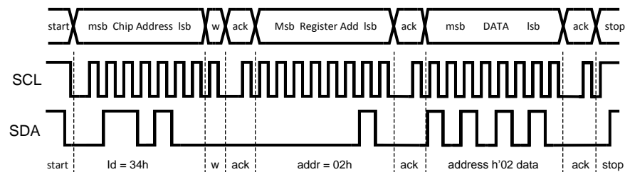
Figure 20. Write cycle
