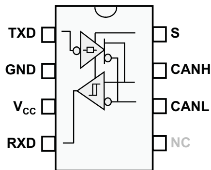
Figure 3. SN65HVD255 Basic Block Diagram & Pin Out
