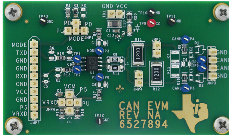
Figure 1. EVM PC Board
