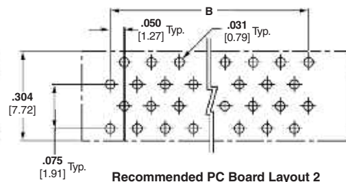
Recommended PC Board Layout 2
