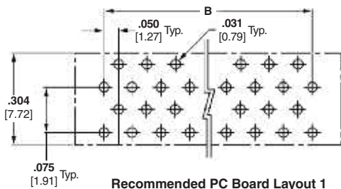
Recommended PC Board Layout 1
