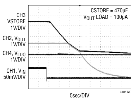
Running on Storage Capacitor
