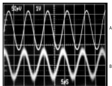
MAX517/MAX519 REFERENCE FEEDTHROUGH AT 100kHz
