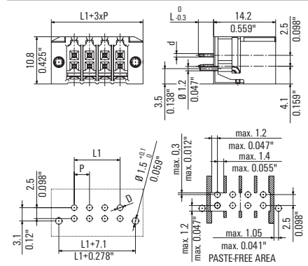
Dimensioned drawing
