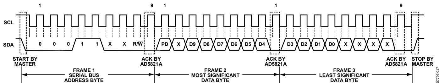
Figure 22. Write Operation
