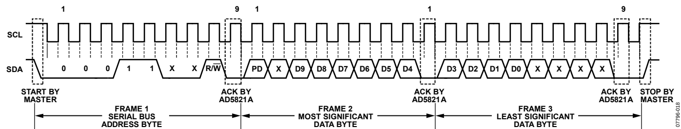
Figure 23. Read Operation
