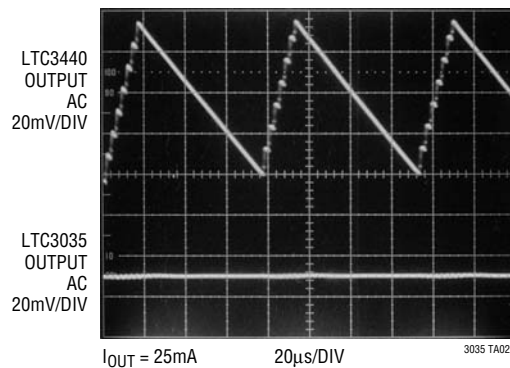
Ripple Rejection
