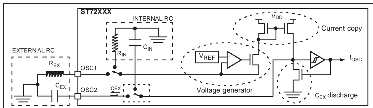
Figure 73. Typical Application with RC oscillator
