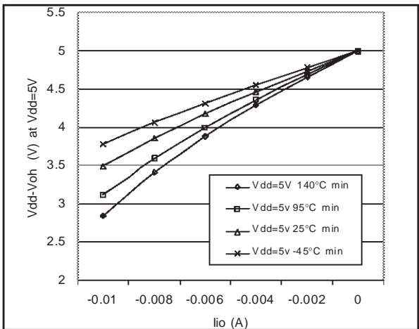
Figure 87. Typical V_{DD}-V_{OH} at V_{DD}=5V
