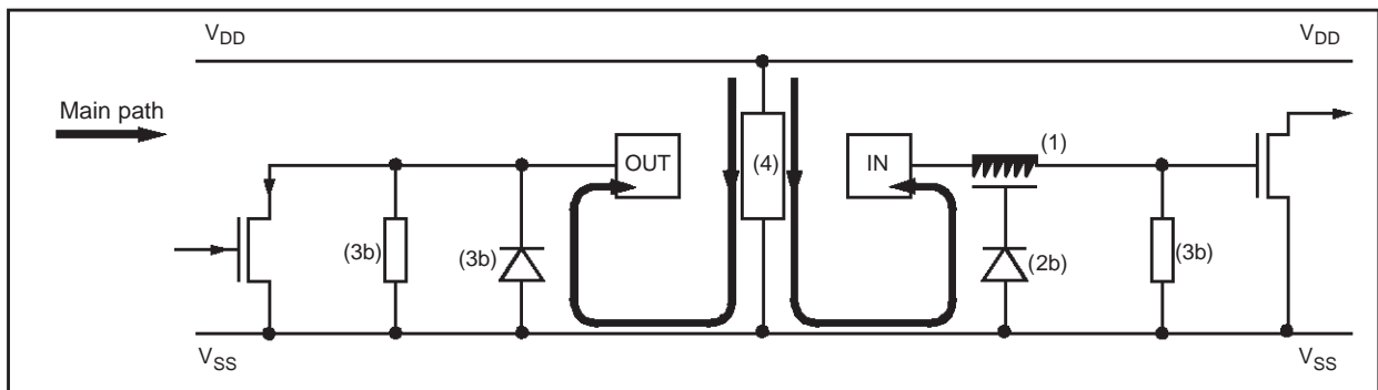
Figure 82. Multisupply Configuration
