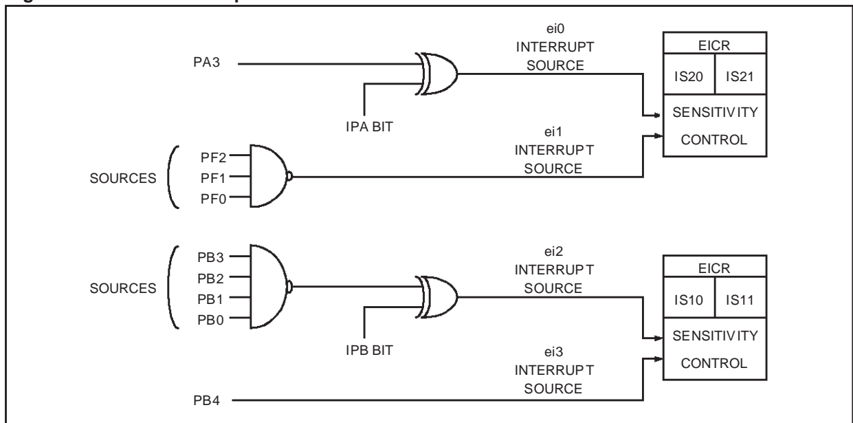
Figure 22. External Interrupt Control bits
