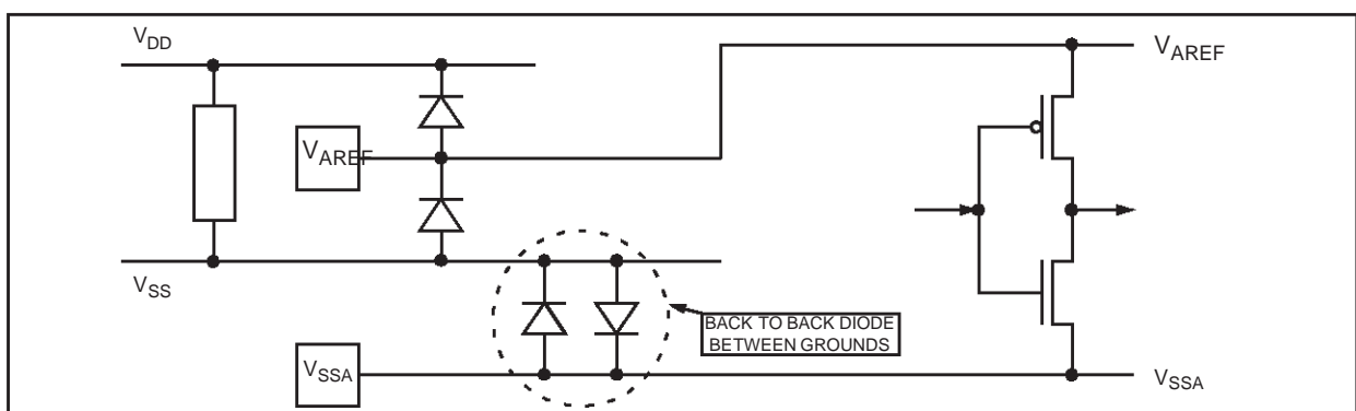
Figure 82. Multisupply Configuration
