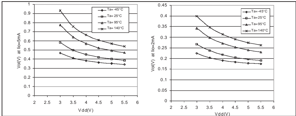
Figure 89. Typical V_{OL} vs. V_{DD} (high-sink)
