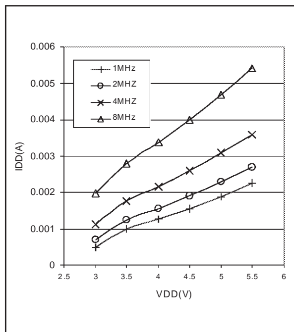
Figure 69. Typical I_{DD} in WAIT vs. f_{CPU}
