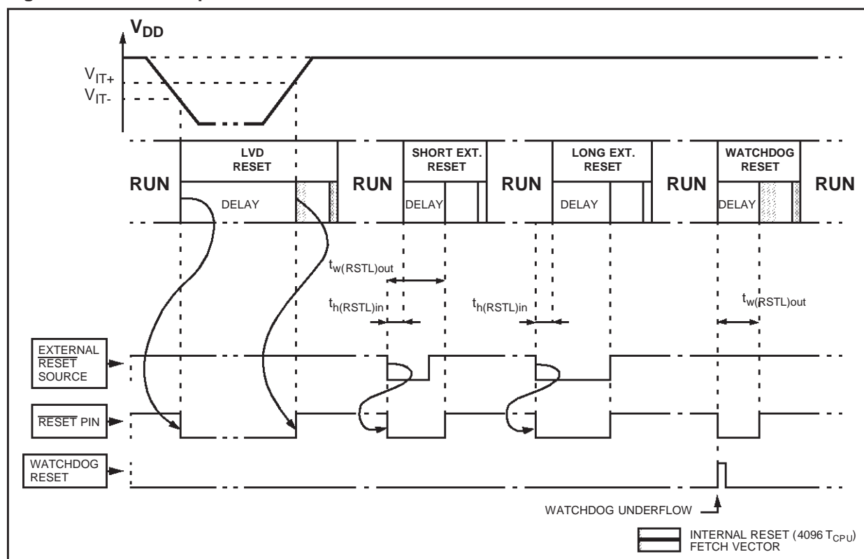
Figure 14. RESET Sequences
