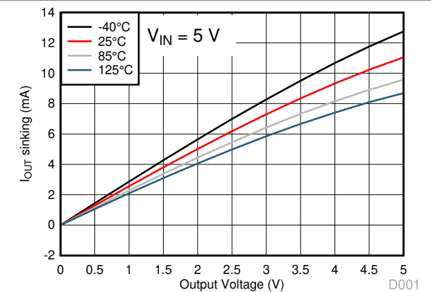
Figure 6-6. Output Discharge Current vs Output Voltage
