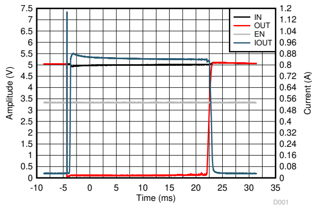
Figure 6-3. Pulsed Output Short
