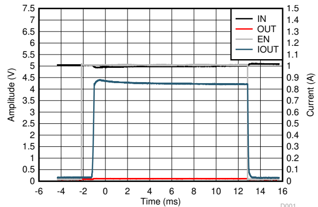
Figure 6-2. Enable into Short
