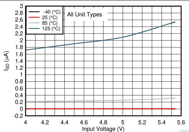
Figure 6-11. Disabled Supply Current ( I_{SD} ) vs Input Voltage
