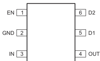
Figure 5-1. DBV Package 6-Pin SOT-23 Top View
