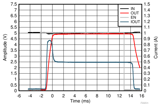
Figure 6-1. Turn ON into 10 \Omega
