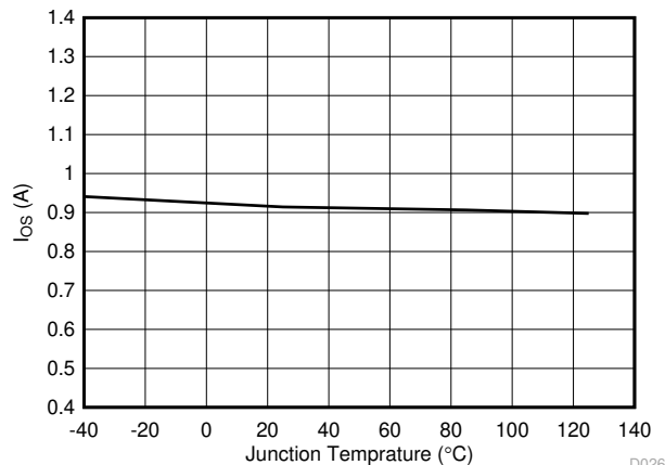
Figure 6-7. Short Circuit Current ( I_{OS} ) vs Temperature
