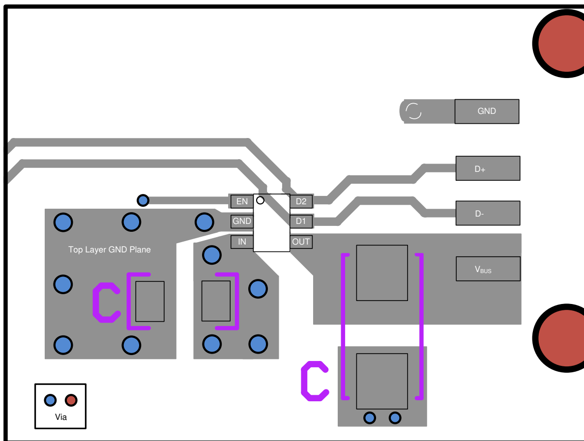
Figure 11-1. USB2.0 Type A TPD3S014-Q1 Board Layout
