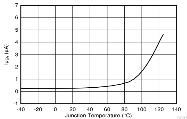
Figure 6-5. Reverse Leakage Current ( I_{REV} ) vs Temperature
