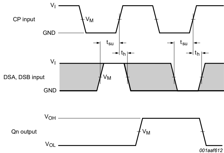
Measurement points are given in Table 8 . The shaded areas indicate when the input is permitted to change for predictable output performance. V_{OL} and V_{OH} are typical voltage output levels that occur with the output load.
