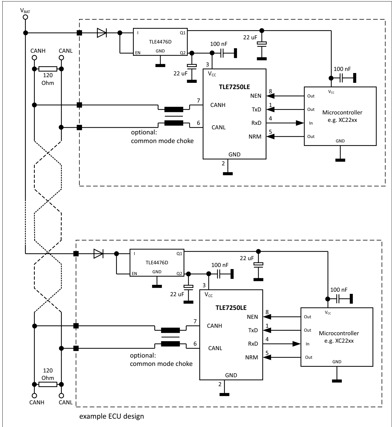
Figure 12 Application circuit
