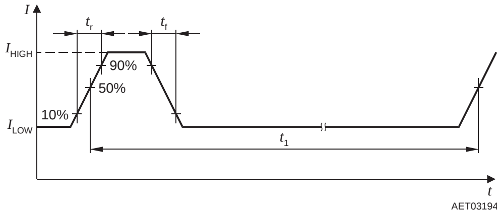
Figure 6 Definition of Rise and Fall Time
