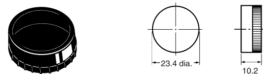
Color Cap A22L-30T □
