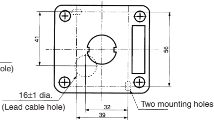
Cable Port Hole (Top View)
