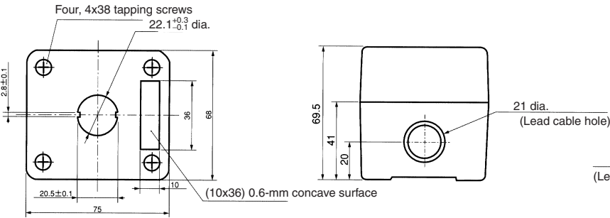
Cable Port Hole (Top View)
