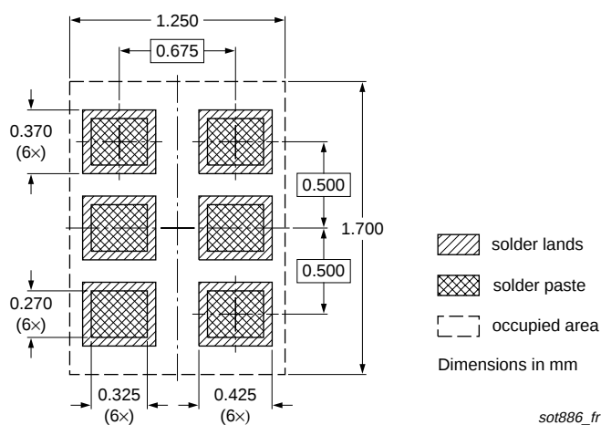
Fig 11. Reflow soldering footprint PESDxS4UF (SOT886)
