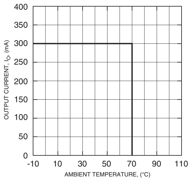
DERATING CHARACTERISTICS
