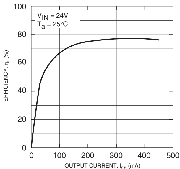
EFFICIENCY VS. OUTPUT CURRENT CHARACTERISTICS
