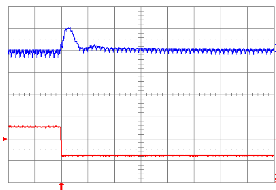
Fig. 1.2V.8: Output voltage response for V_{out} = 1.2V to a negative load current step change from 5A to 2.5A with a slew rate of 5A/\mu s at V_{in} = 12V . Top trace: output voltage (100mv/div); Bottom trace: load current (2A/div). C_o = 47\mu F ceramic. Time scale: 20 \mu s /div.
