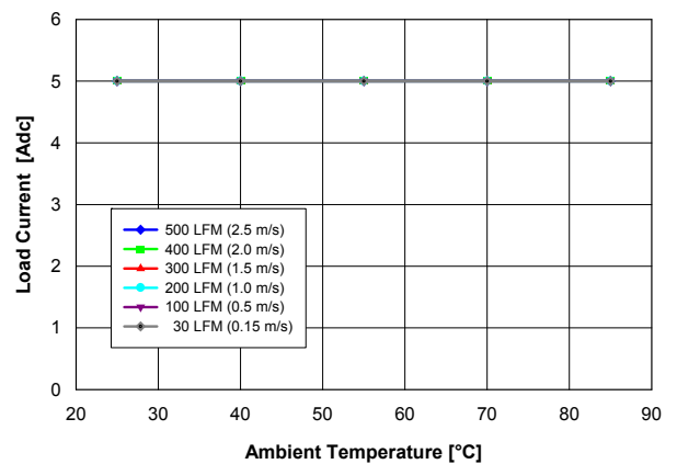
Fig. 2.0V.2: Available load current vs. ambient temperature and airflow rates for V out = 2.0V converter mounted horizontally with V in = 12V, air flowing from pin 5 to pin 1 and maximum MOSFET temperature ≤ 120 °C.
