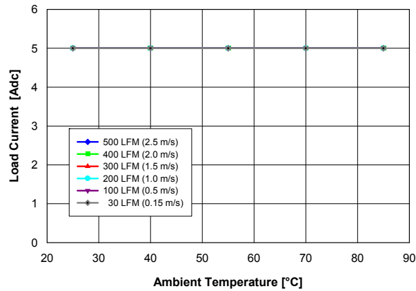
Fig. 2.0V.1: Available load current vs. ambient temperature and airflow rates for V out = 2.0V converter mounted vertically with V in = 12V, air flowing from pin 5 to pin 1 and maximum MOSFET temperature ≤ 120 °C.
