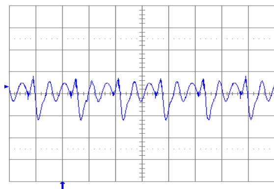
Fig. 1.2V.6: Output voltage ripple (10mv/div) at full rated load current into a resistive load with external capacitance 47\mu F ceramic + 1\mu F ceramic and V_{in} = 12V for V_{out} = 1.2V . Time scale: 2 \mu s /div.
