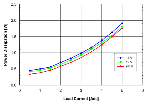
Fig. 2.0V.4: Power Loss vs. load current and input voltage for V out = 2.0V converter mounted vertically with air flowing from pin 5 to pin 1 at a rate of 200 LFM (1 m/s) and T a = 25 °C.
