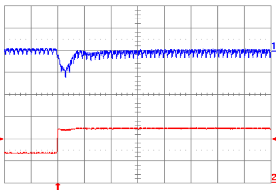
Fig. 1.5V.7: Output voltage response for V_{out} = 1.5V to a positive load current step change from 2.5A to 5A with a slew rate of 5A/\mu s at V_{in} = 12V . Top trace: output voltage (100mv/div); Bottom trace: load current (2A/div). C_o = 47\mu F ceramic. Time scale: 20 \mu s /div.
