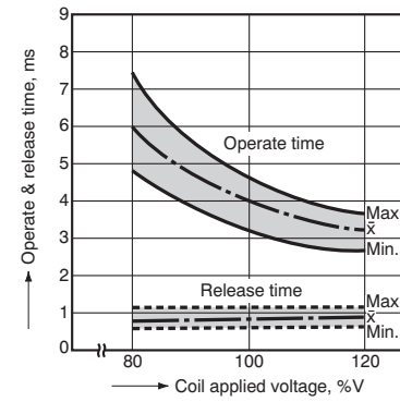
4.-(6) Operate & release time (with diode, 2 Form A) Tested sample: DSP2a-DC12V, 5 pcs.
