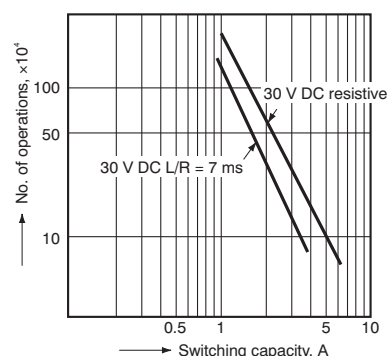
2.-(2) Life curve (1 Form A 1 Form B)
