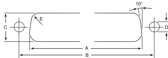
Rear Mounting Cutout
