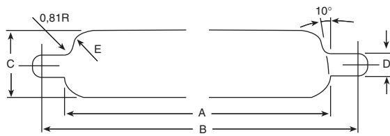
Front Mounting Cutout
