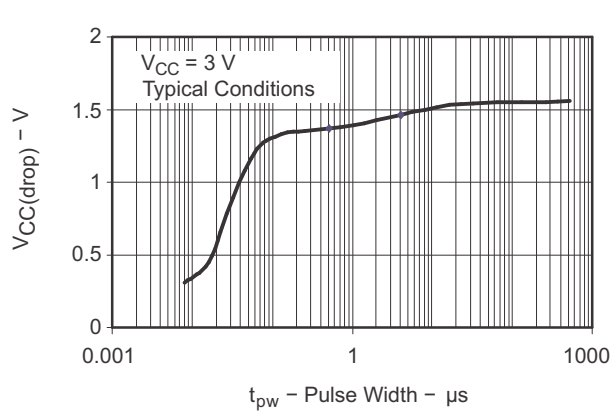
Figure 9. V_{CC(drop)} Level With a Square Voltage Drop to Generate a POR or BOR Signal
