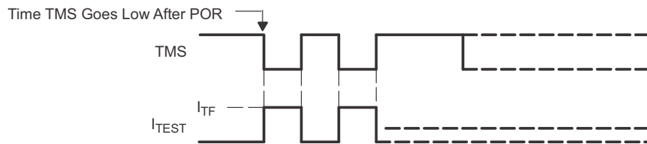
Figure 23. Fuse Check Mode Current
