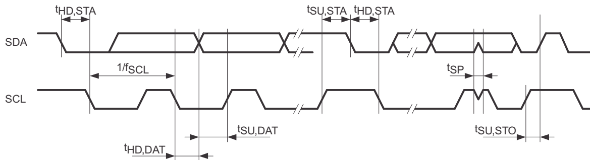
Figure 22. I2C Mode Timing
